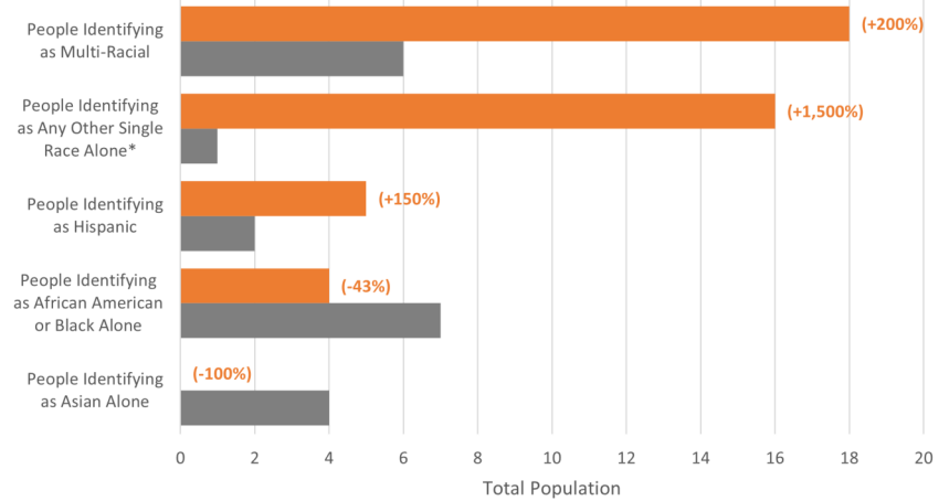
Changing Diversity in Lincoln Borough Change in Selected Racial & Ethnic Demographic Populations 2010 to 2020
